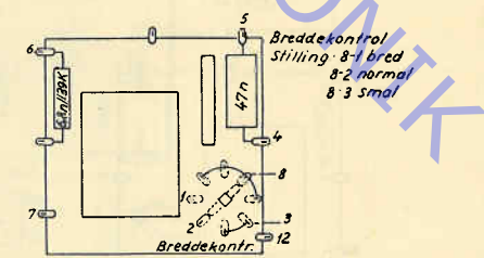
Linieuangangstransfomator. AT 2010
